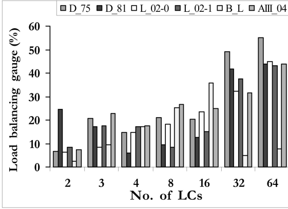
Fig. 9. Load balancing gauge ( \Delta_{FE} ) versus \Psi under \beta = 4K and \gamma = 50 percent.
