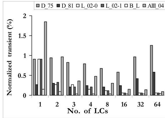
Fig. 12. Normalized transient versus \Psi under \beta = 4K and \gamma = 50 percent.
