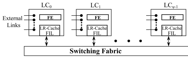
Fig. 1. A SPAL-based router, where FIL refers to fabric interface logics.
