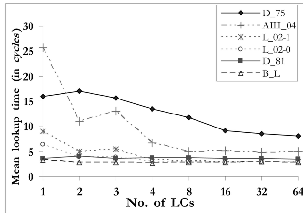
Fig. 8. Mean lookup time (in cycles) versus \Psi under \beta = 4K and \gamma = 50 percent.
