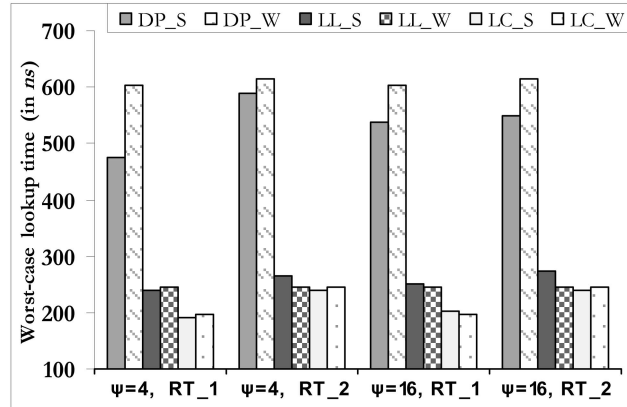
Fig. 5. Worst-case lookup time (in ns) under cycle time = 5 ns and SRAM access time = 12 ns.
