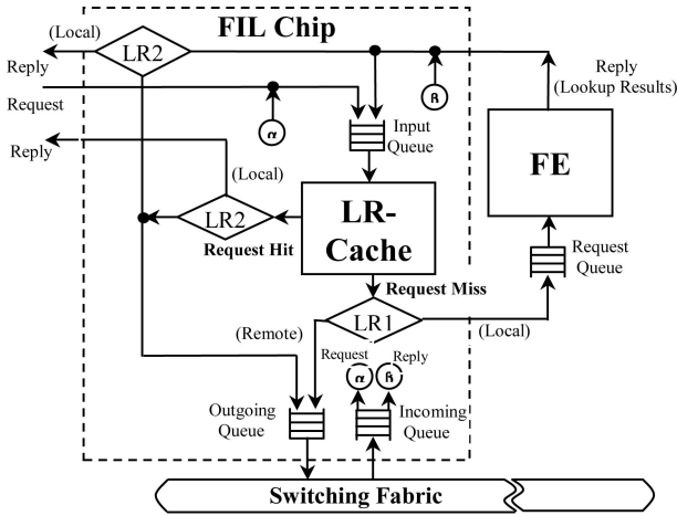
Fig. 3. LR-cache and relevant logics housed inside the FIL chip, where an LR1 (or LR2) detector examines the destination (or originator) address.
