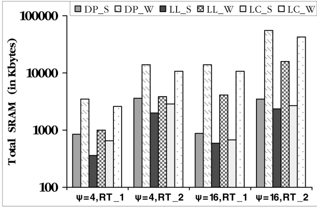
Fig. 4. Total SRAM (in Kbytes) required for different tries under IPv4.
