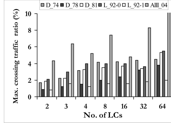
Fig. 10. Maximal crossing traffic ratio (percent) versus \Psi under \beta = 4K and \gamma = 50 percent.
