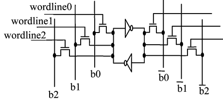
Fig. 11. A multiport SRAM cell.
