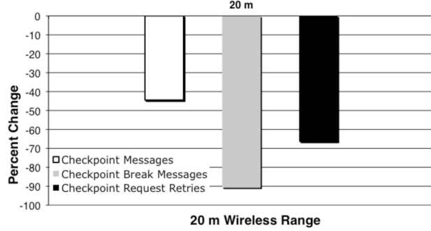
Fig. 8. ReD versus RCA in testbed message percent change.
