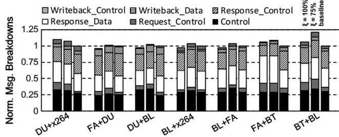
Fig. 8. Normalized NoC message breakdowns (w.r.t. those of the baseline shown in the rightmost bar of each workload mix) under multitasking with equal domain partitioning for 64 cores, with \xi = 100\% (or 75 percent) denoted in the leftmost (or middle) bar of each workload.
