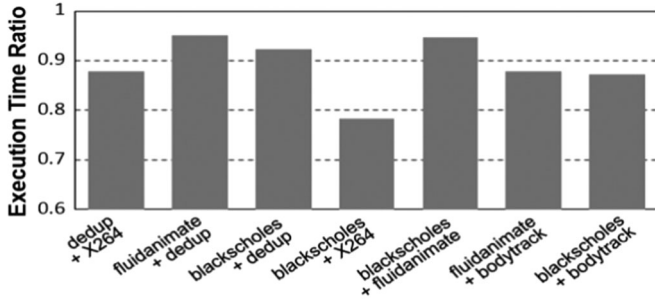
Fig. 1. Execution time results for two PARSEC benchmarks executed simultaneously on 64 cores, denoted by the ratios of those under domain partitioning against those without partitioning, where benchmarks are detailed in Table 2.
