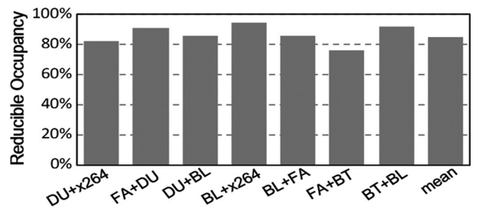
Fig. 4. Reducible occupancy in SPT for 64 cores under multitasking with threads pinned to cores.
