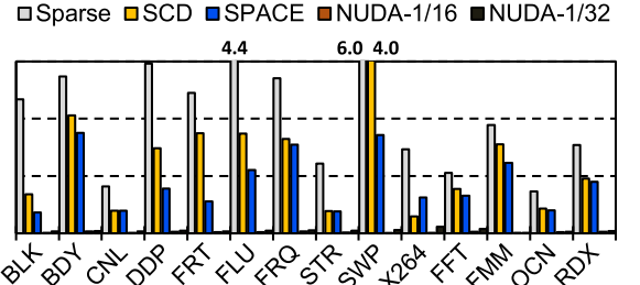
Fig. 12. Normalized execution times of NUDA and its earlier counterparts with respect to those of FBM, with the coverage of Sparse, SCD, and SPACE all equal to 1/16.
