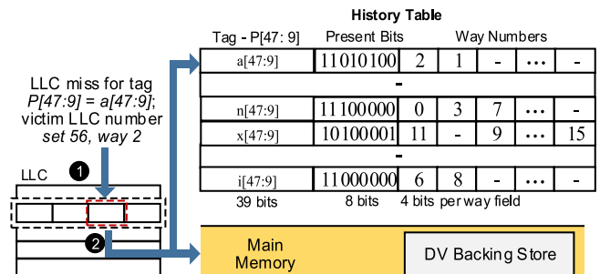
Fig. 6. Memory block access history table kept in each memory controller for PAVE. Each history table entry includes a tag field, an 8-bit presence field, and eight way-fields, where the tag field keeps the first 39 bits of the 48-bit physical address, aligned at (8 \times 64) for the cache block size of 64 bytes.
