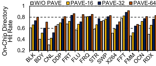
Fig. 10. On-chip directory hit rates under various prefetching buffer sizes for NUDA-1/16.
