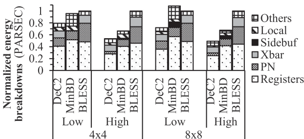
Fig. 7. Network energy breakdowns under PARSEC benchmark traces, with results all normalized against those of BLESS under 4 \times 4 and 8 \times 8 mesh-based NoCs.
